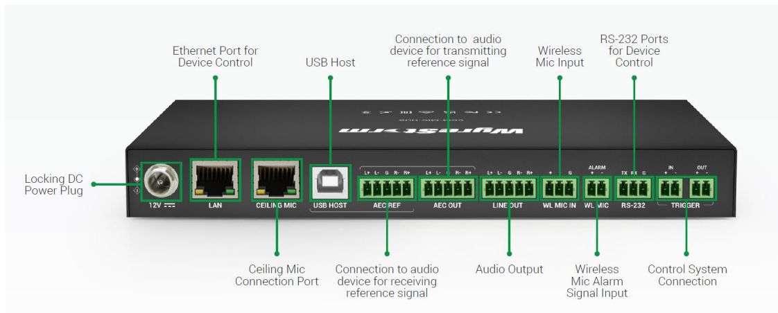
Rear Panel
